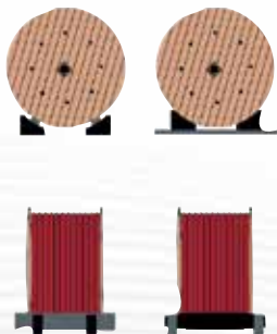
Secure the drums firmly
