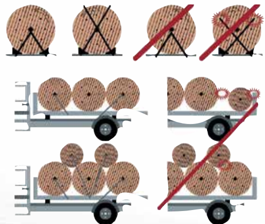
Fasten the drums firmly
